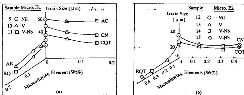
Figure 1. Austenite grain size after casting, rolling and heat treatment of steel (a) samples 9 to 11 and (b) samples 12 to 15.
