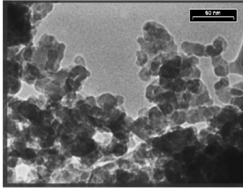
Fig. 1. TEM picture of \text{Al}_2\text{O}_3 nanopowders (35nm).
